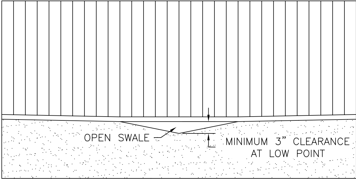
PROPER FENCE CONSTRUCTION
